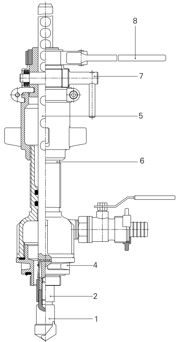
FIG. 3 Drilling machine assembly with drill bit for cast pipes
